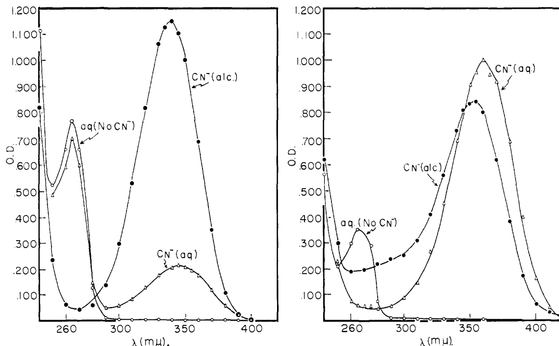
Fig. 1.—The aqueous and methanolic potassium cyanide addition reactions: 0.19 \mu mole of 1-methyl nicotinamide iodide (or 1-methyl-3-acetylpyridinium iodide) was treated with molar potassium cyanide (aq.) or saturated potassium cyanide (methanol) (final volume 3.0 ml.; 25°).
