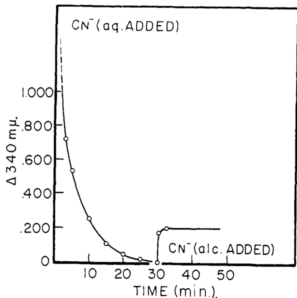
Fig. 2.—Hydrolysis of 1-methyl-3-ethoxycarbonyl pyridinium iodide: 1.0 \mu mole of 1-methyl-3-ethoxycarbonyl pyridinium iodide was treated with potassium cyanide (0.3 M final concentration) in a solution buffered with 0.5 M potassium phosphate (final volume 3.0 ml.; final pH 10.7; 25°). After 30 minutes 5 ml. of saturated methanol-potassium cyanide was added to the mixture (no correction made for the dilution factor). A 3-ml. aliquot was extracted and the change in optical density with time was measured at 330 m\mu . Concentration of 1-methyl-3-ethoxycarbonylpyridinium iodide 0.2 \mu M .
