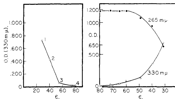
Fig. 3a.—Potassium cyanide addition as a function of dielectric constant: solvents of various dielectric constant. 0.37 \mu mole of trigonelline was treated with molar potassium cyanide. The following solvents are employed: water ( \epsilon = 80.1 ; point 4), methanol-water ( \epsilon = 40.4 ; point 2), ethanol-water ( \epsilon = 55.0 ; point 3) and a dioxane-water mixture ( \epsilon = 29.2 ; point 1).
